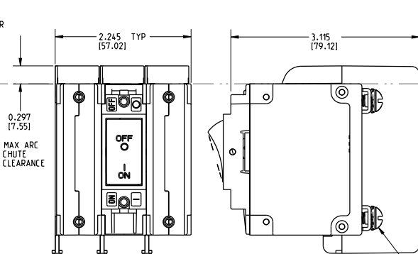
3-POLE (CC3,CD3) w/ ARC CHUTE BARRIER
