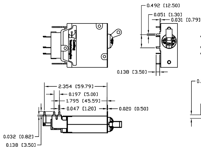
PRINTED CIRCUIT BOARD MOUNTING TERMINAL CODE R
